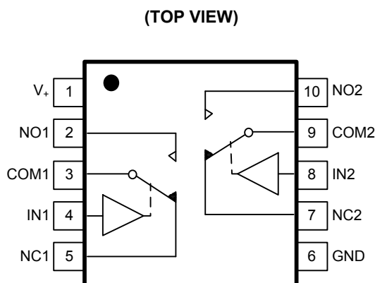
MSOP-10
